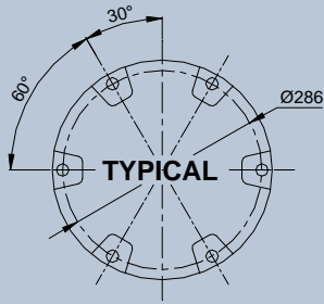
TYPICAL Light Fixture 12" dia.
